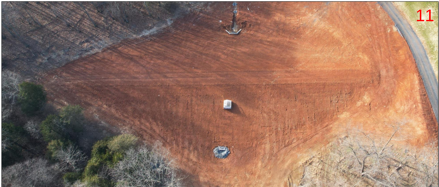
Outlet Structure and embankment overview
